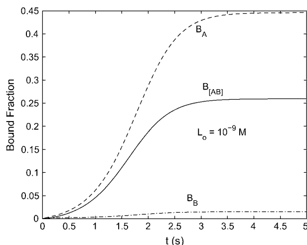
FIGURE 10 Bridging device with \gamma = 0.005 : B_A is the fraction of singly-bound A-analyte, B_B is the fraction of singly-bound B-analyte, and B_{[AB]} is the fraction of doubly-bound (crosslinked) analyte.
